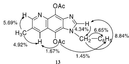
Figure 3. ^1\text{H} NMR NOE DIFF experiments performed on 13 .
