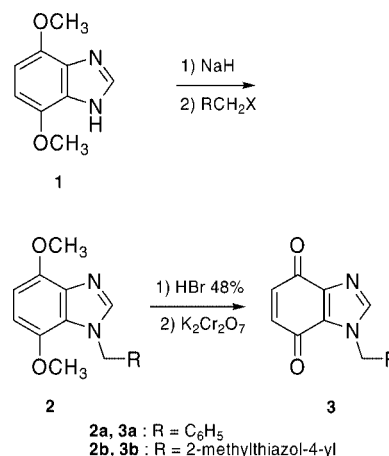
Scheme 1. Synthesis of benzimidazolidione derivatives 3 .
