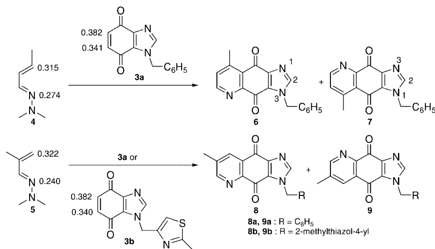
Scheme 2. Synthesis of imidazoquinolinediones 6–9 .
