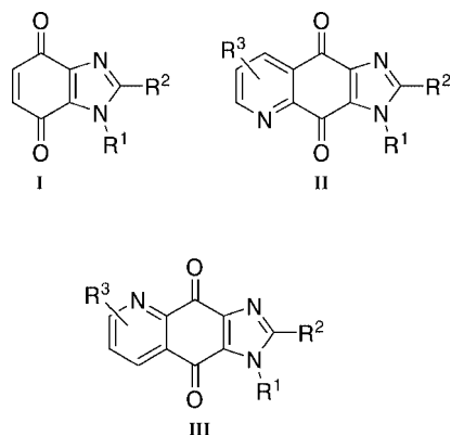
Figure 1. Benzimidazolidiones I and imidazoquinolinediones II–III .
