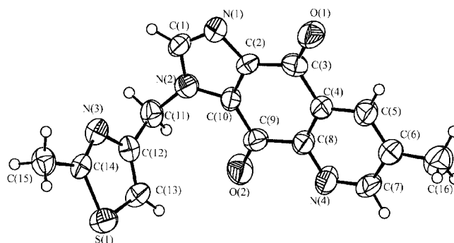
Figure 2. X-ray crystal structure of 8b (anisotropically refined atoms shown as 50% displacement ellipsoids).
