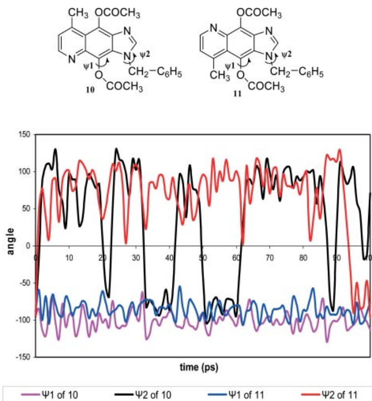
Figure 4. Plotting of dihedral angle ( \psi ) values vs. time for compound 10 and 11 during molecular modelling simulation.
