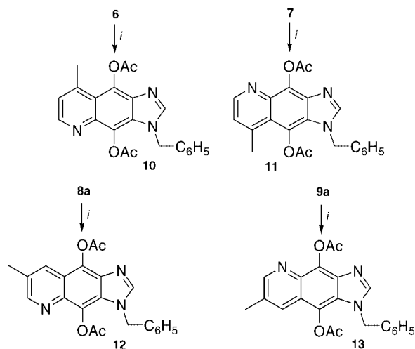
Scheme 3. Synthesis of the diacetoxy derivatives of compounds 6 , 7 , 8a , 9a . (i): \text{Ac}_2\text{O} , \text{Zn}/\text{AcONa} .
